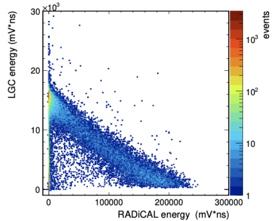
Fig. 8. Integrated signals (mV · ns) in the LGC versus integrated low-gain signals in the RADiCAL module for 28 GeV beam.
